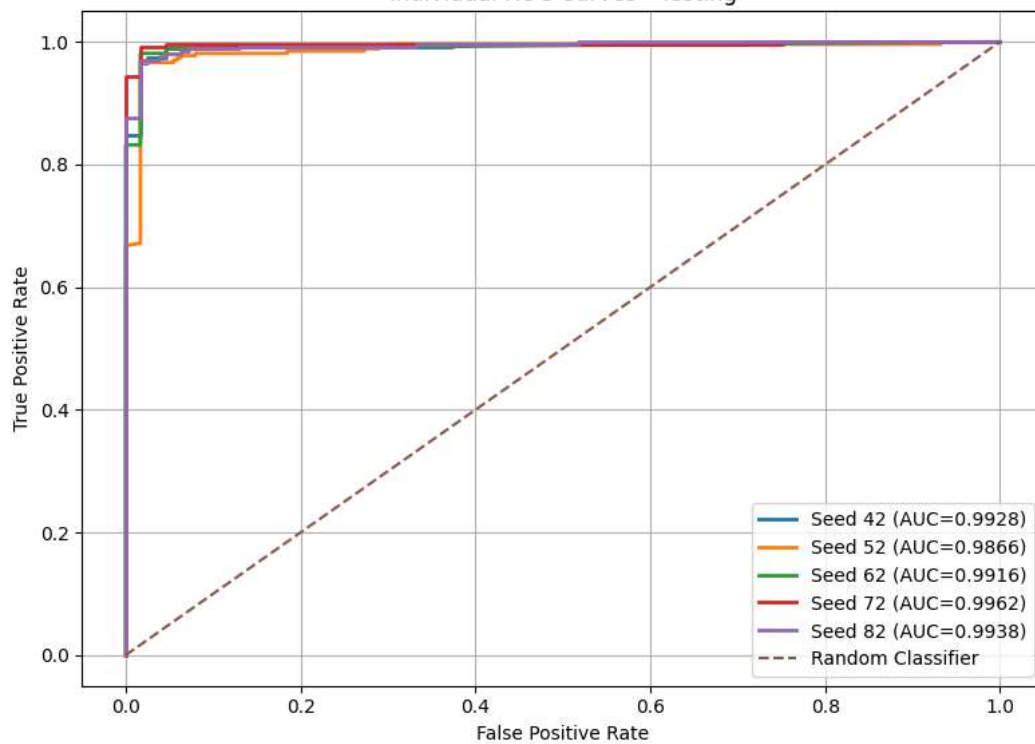
Individual ROC Curves - Testing
