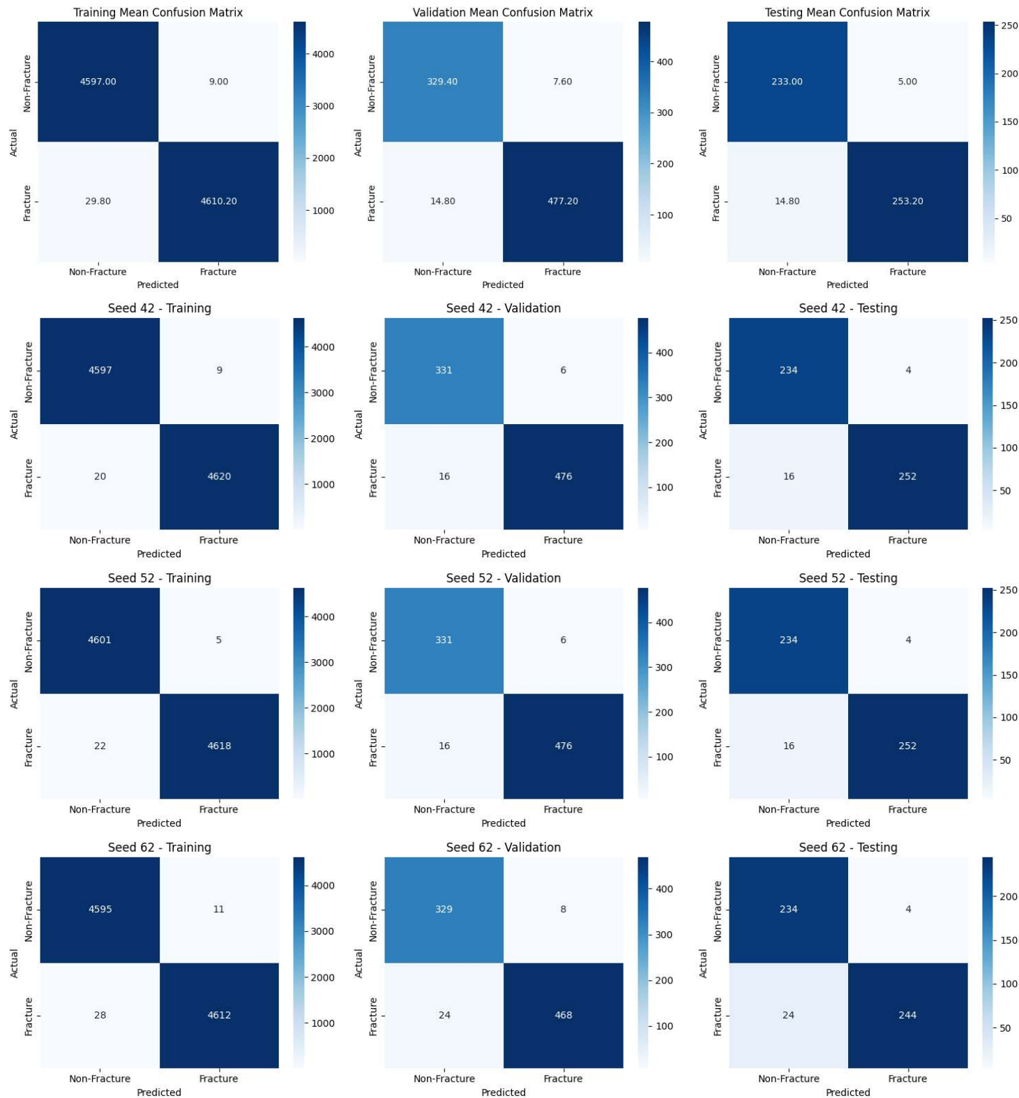
Mean Confusion Matrices Across Five Seeds
