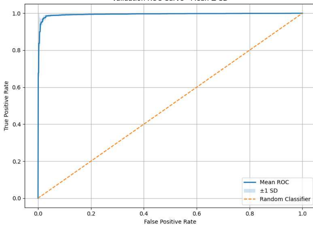
Validation ROC Curve - Mean \pm SD
